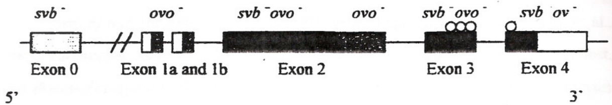
ovo Locus Containing svb and ovo genes
